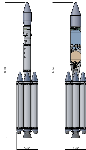
VLS-1 and VLS-1B
