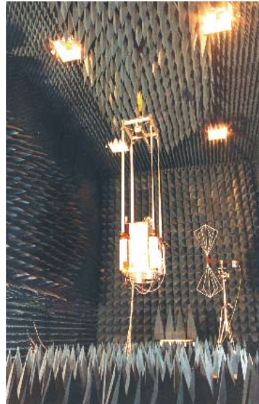
Anechoic chamber, LIT
